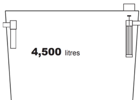
Single chamber septic tank
